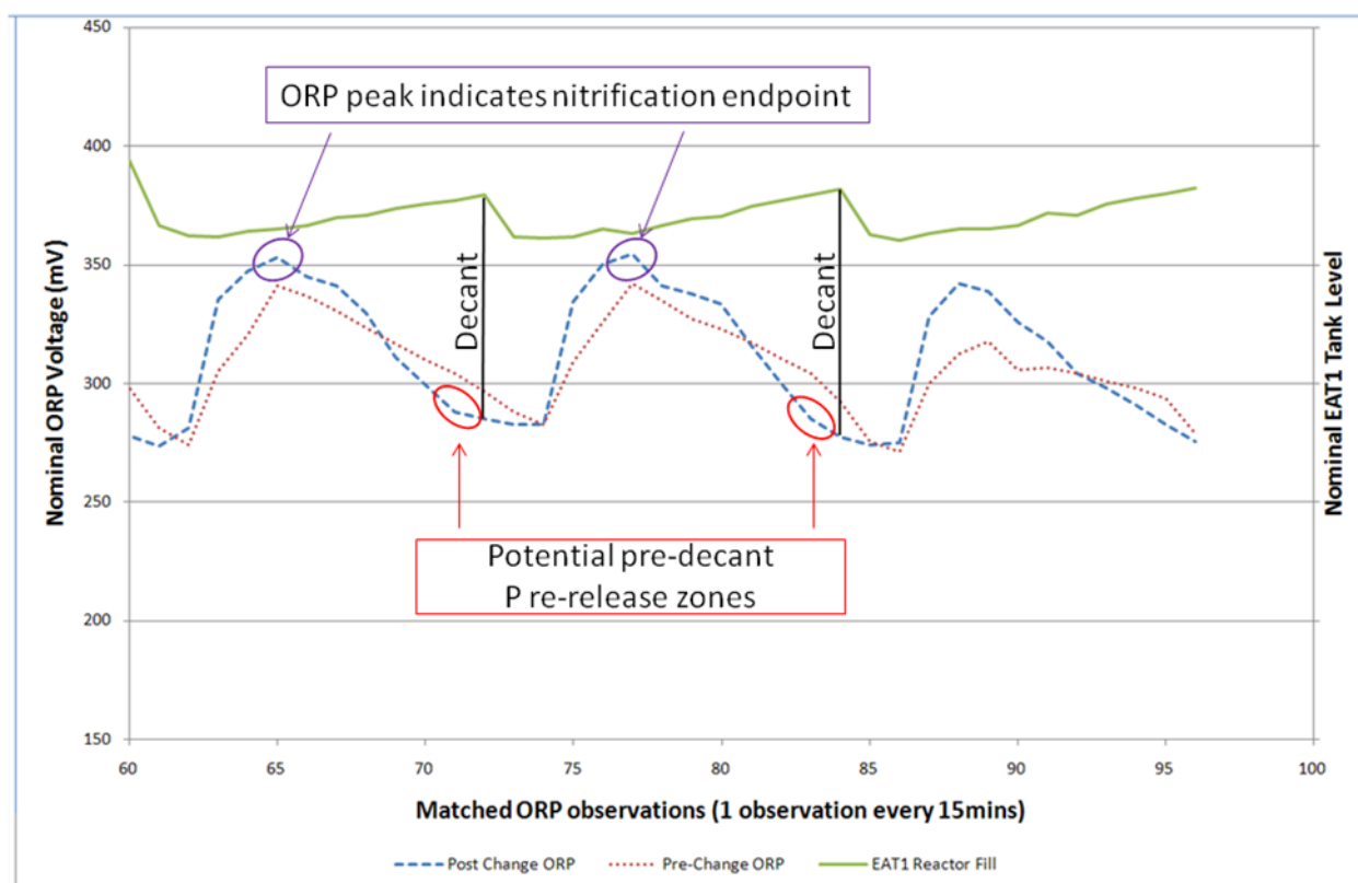
Figure 3-3: A comparison of pre and post change normalized ORP trends
