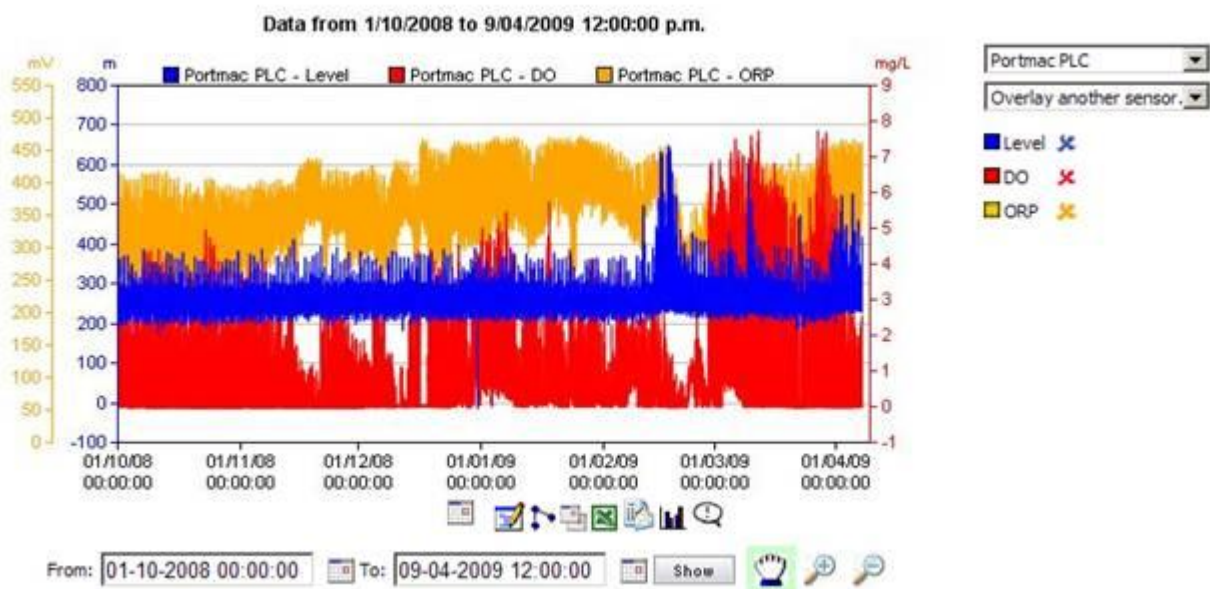
Figure 2-2 Port Macquarie EAT1 telemetered DO, ORP, and level data
