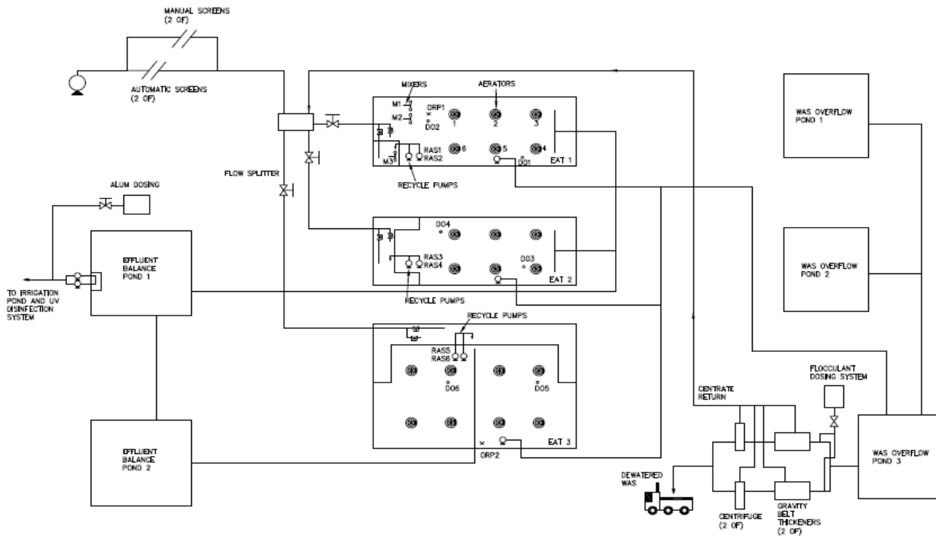
Figure 1-1: Port Macquarie WWTP General Arrangement
