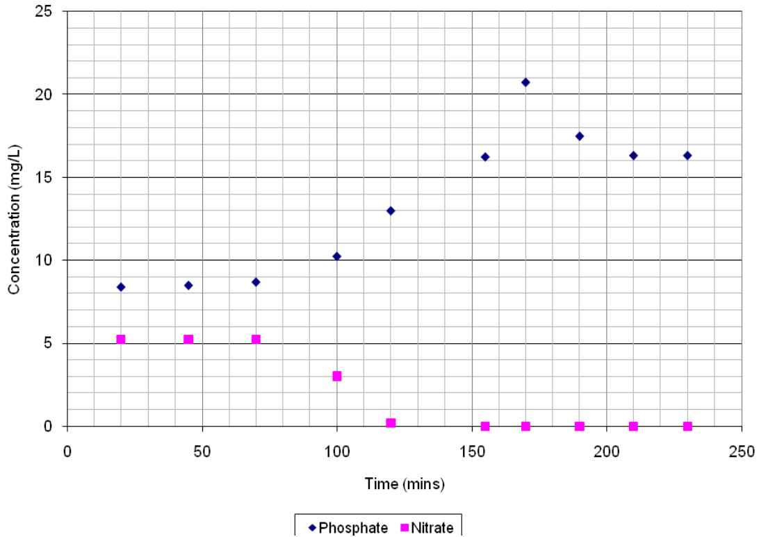
Figure 3-1: Phosphorous Release Rate Tests
